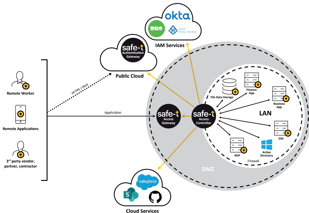
ZoneZero SDP – Classic cloud deployment
